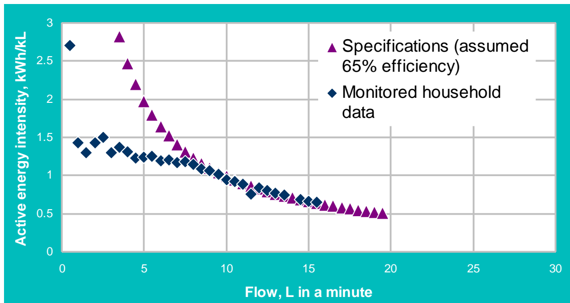
Figure 23: Comparison against specifications for a pump at a single household
